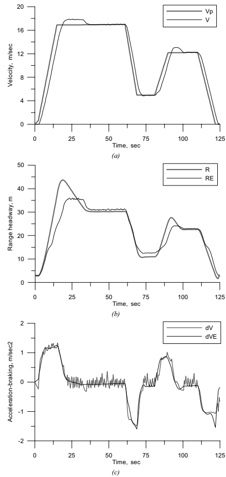
Fig. 5. Driving behavior in longitudinal motion and estimation (a) velocities of both cars, (b) range-clearance: actual (R) and estimated (RE) values, (c) acceleration-braking: actual (dV) and estimated (dVE) values.
